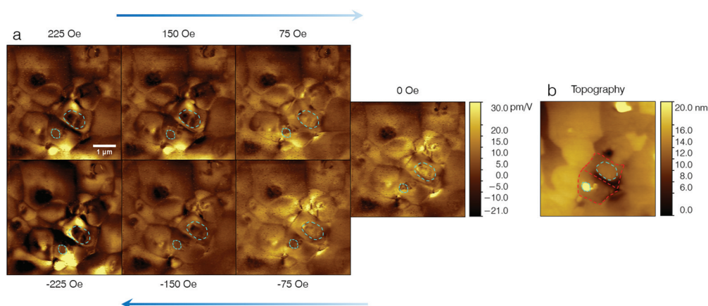
Fig. 5 PFM under in situ lateral magnetic field. (a) VPFM X-Amplitude (mixed signal) images under in situ lateral magnetic field. (b) Topography of the same region as in (a). A CFO core and CFO core/BFO-rich inner shell are marked by cyan dashed circles, while their host grains are marked by red dashed lines. (a). Ramping of magnetic field and order in which images were taken are illustrated by direction of blue arrows. All PFM images have the same contrast scale. Strong changes of the PFM X-Amplitude as a function of the magnetic field occur, which indicates a change of electric polarization as a function of magnetic field.
